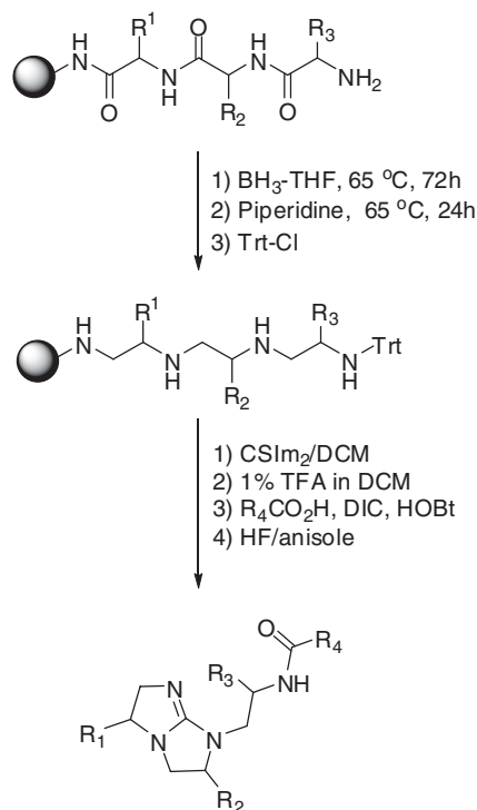
Scheme 1. Synthesis of the N -acylated bicyclic guanidine positional scanning library.
